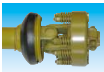
PTO shaft with friction disc slip clutch
